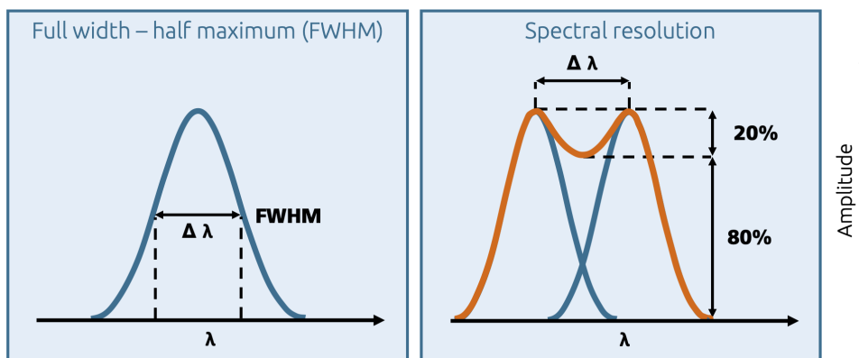
Full width, half maximum (FWHM) and spectral resolution of bands
